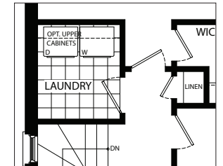
Second Floor 3 Bedroom With Laundry Option Elevation A/B
