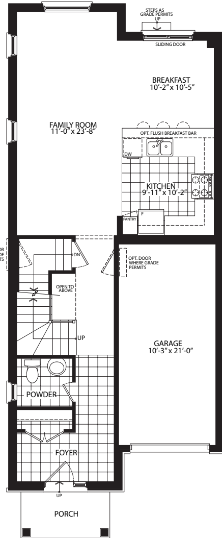
Main Floor Elevation A
