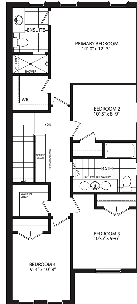
Second Floor With 4 Bedroom Option Elevation A
