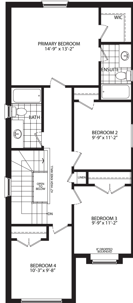
Second Floor With 4 Bedroom Option Elevation A
