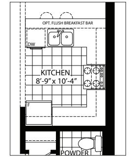
Main Floor With Alternate Kitchen Layout Elevation A/B
